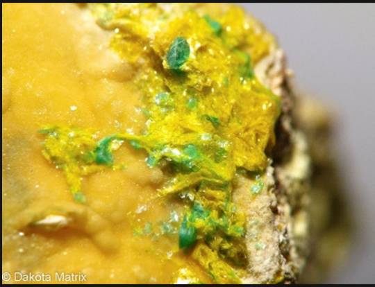
Francoisite-(Nd) - Congo
